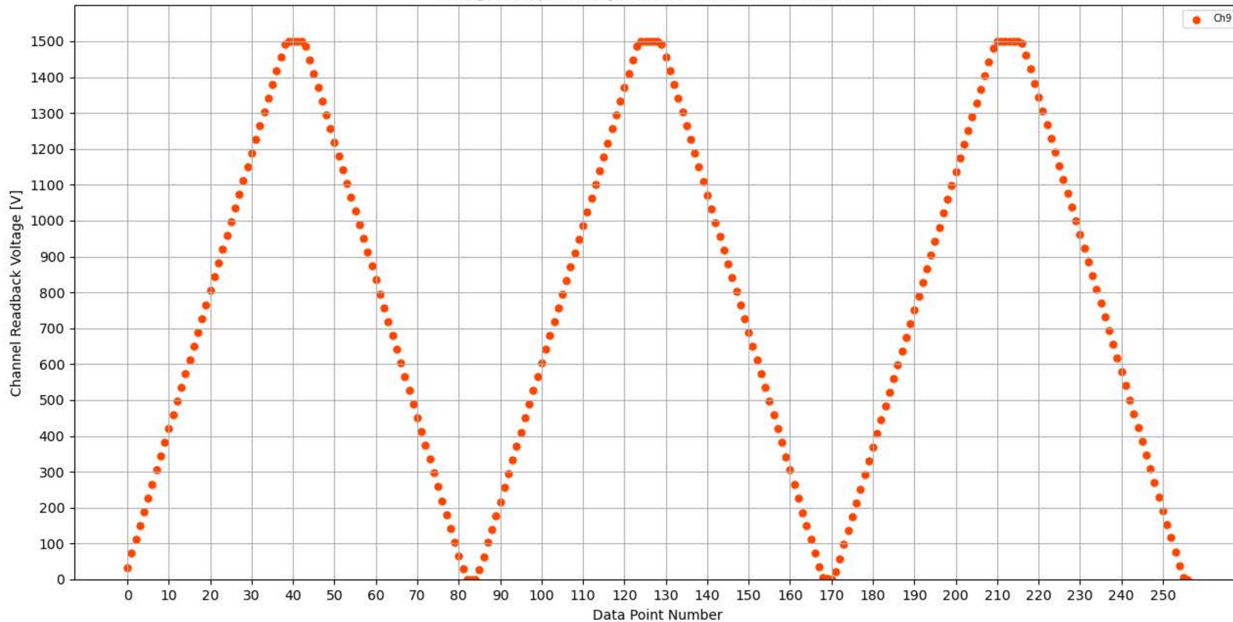
Voltage Ramp Test (Python) Bd #347, Slot #13, Ch #9
