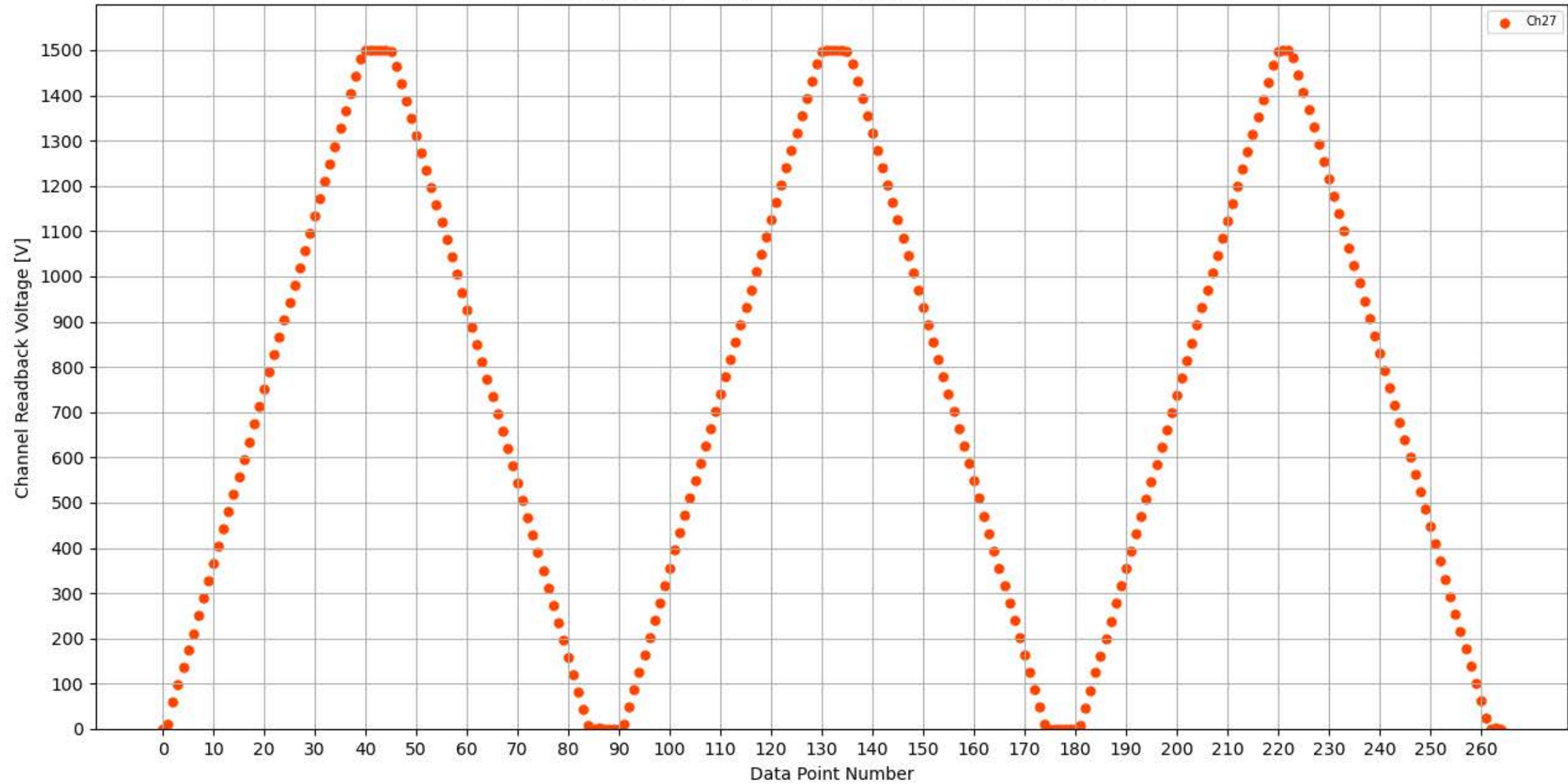
Voltage Ramp Test (Python) Bd #347, Slot #13, Ch #27
