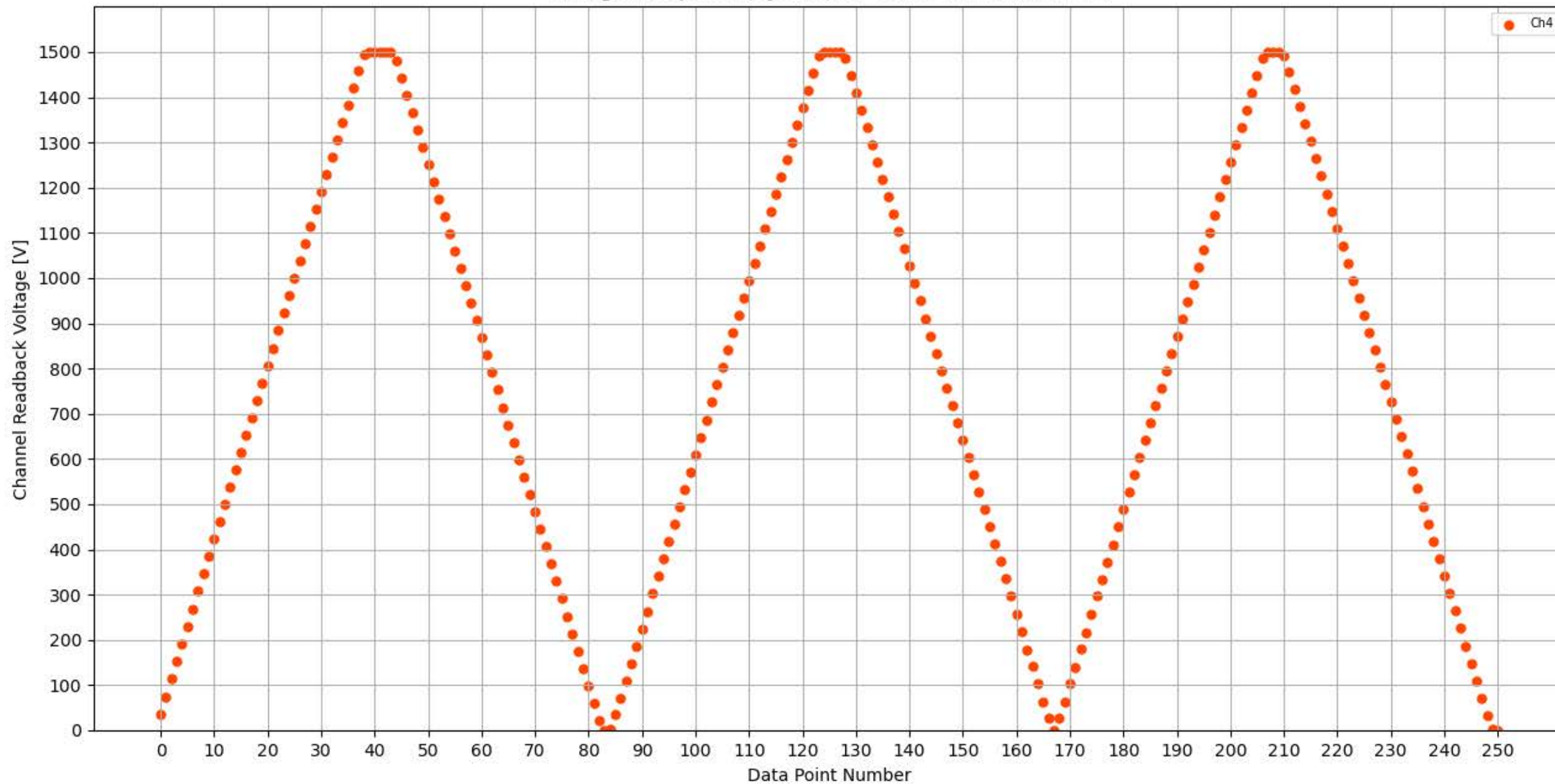
Voltage Ramp Test (Python) Bd #347, Slot #13, Ch #4
