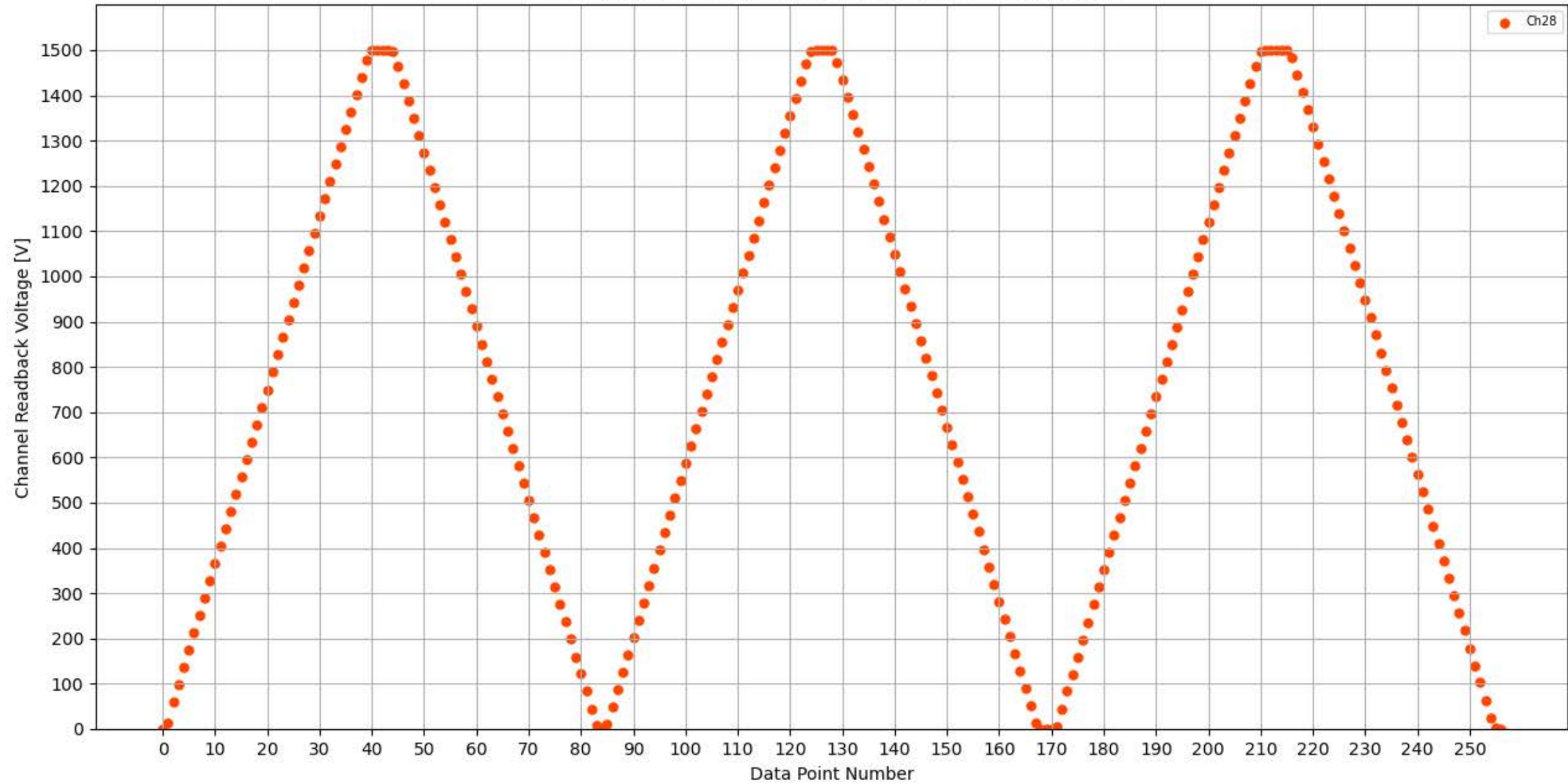
Voltage Ramp Test (Python) Bd #347, Slot #13, Ch #28
