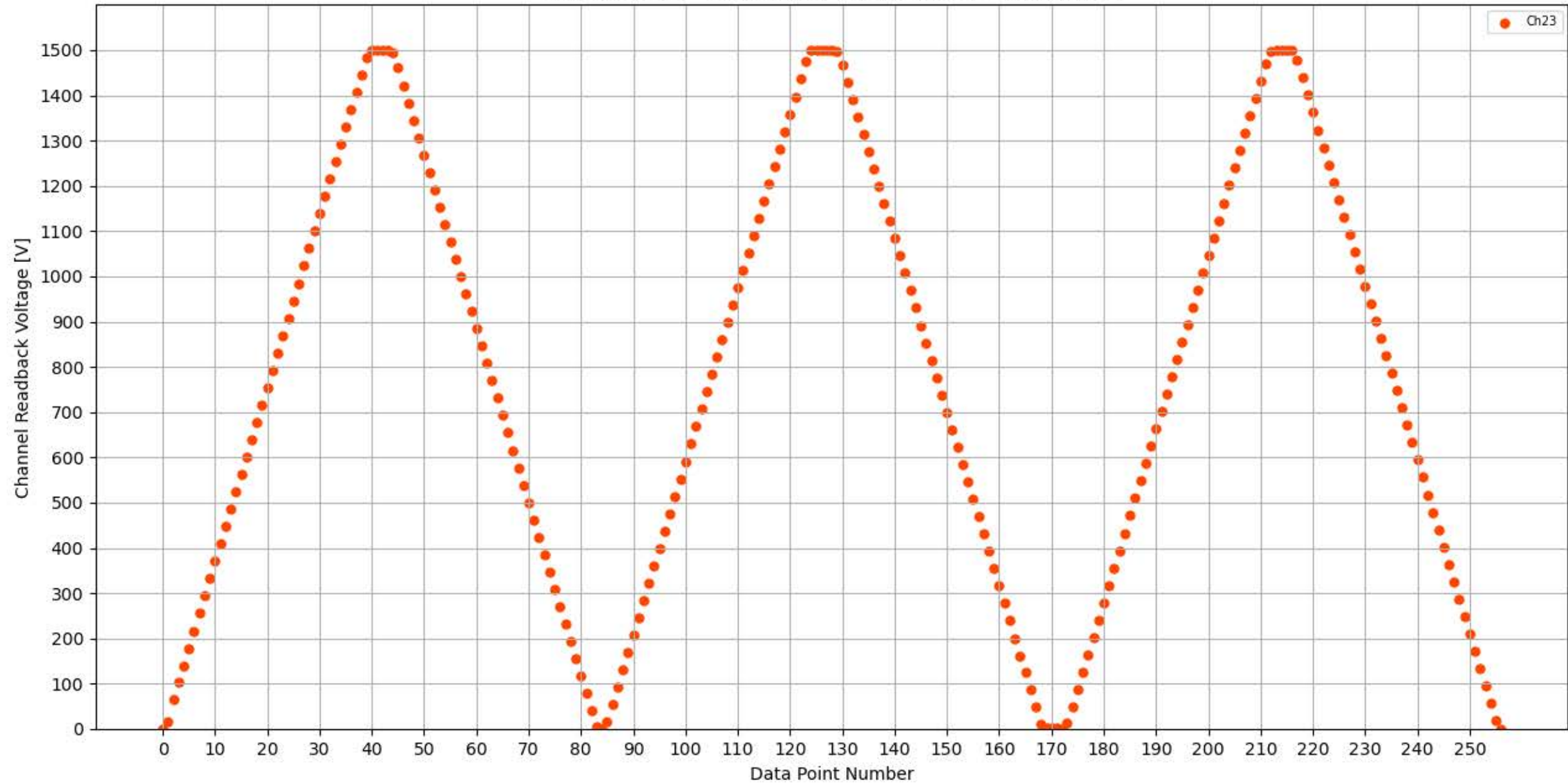
Voltage Ramp Test (Python) Bd #347, Slot #13, Ch #23
