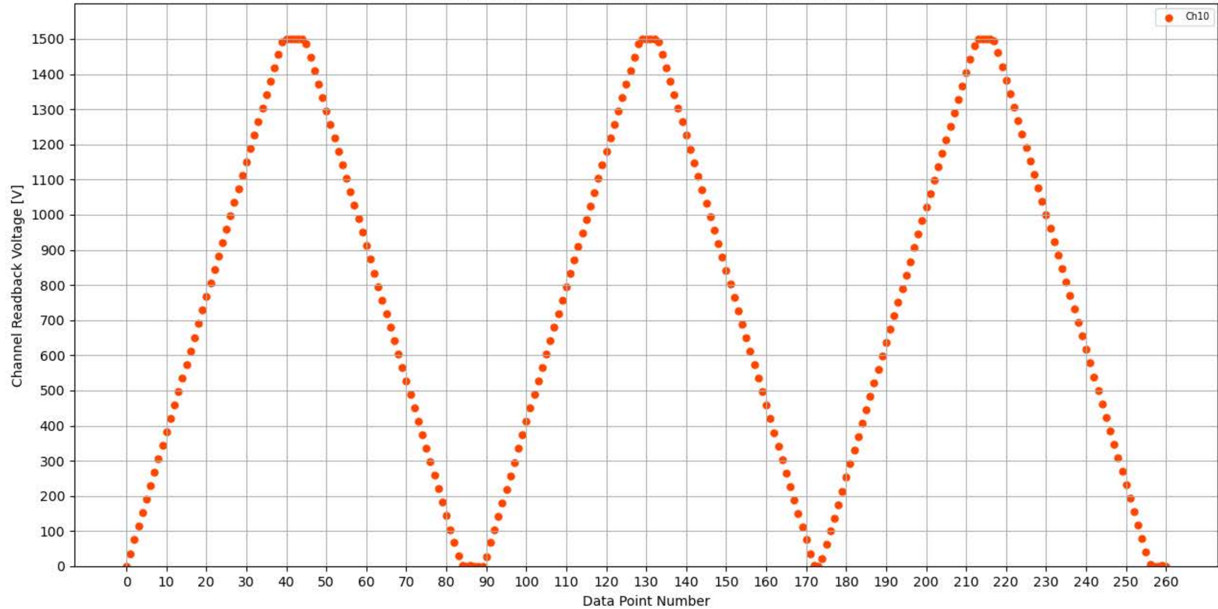
Voltage Ramp Test (Python) Bd #347, Slot #13, Ch #10
