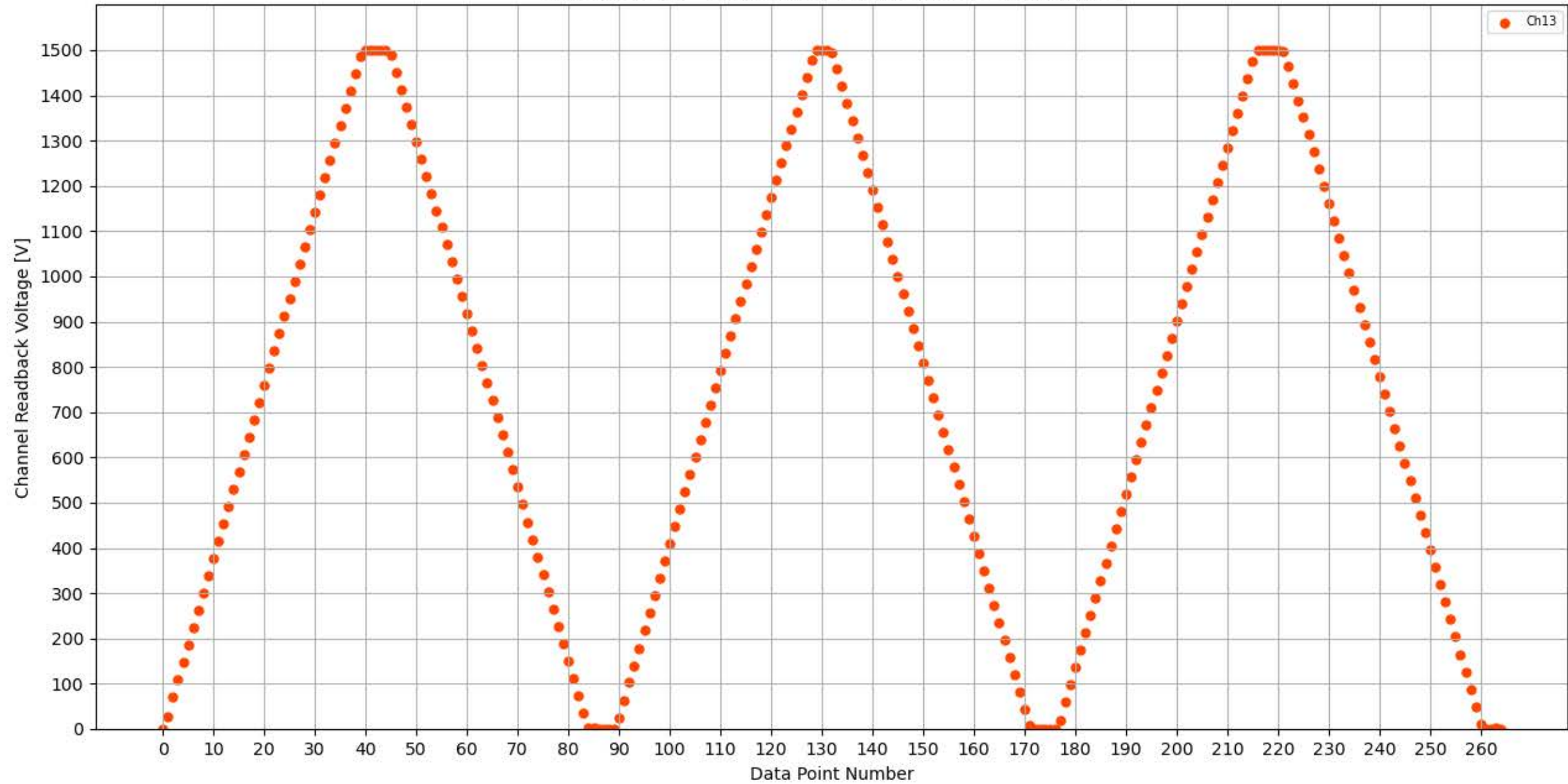
Voltage Ramp Test (Python) Bd #347, Slot #13, Ch #13
