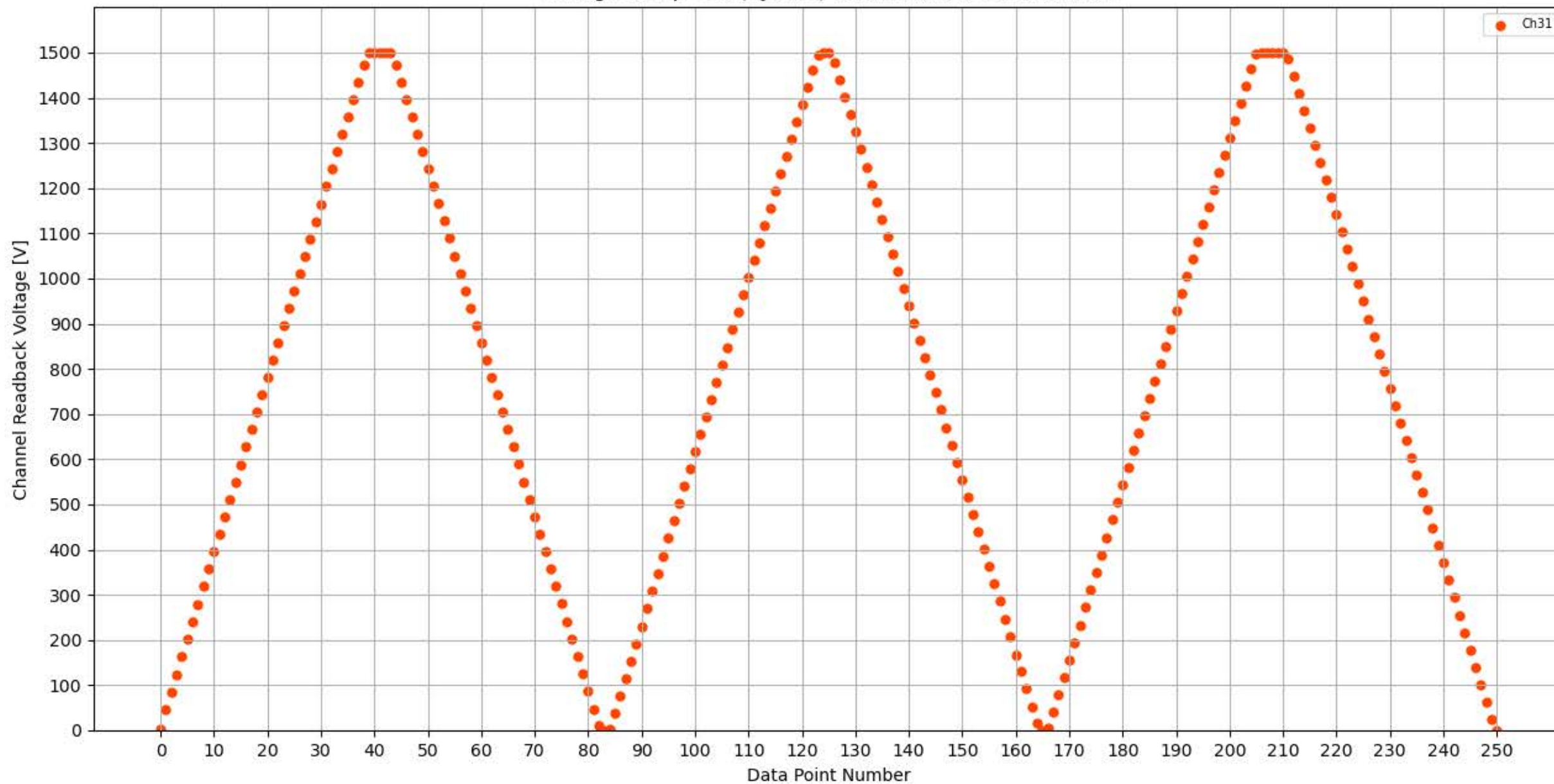
Voltage Ramp Test (Python) Bd #347, Slot #13, Ch #31
