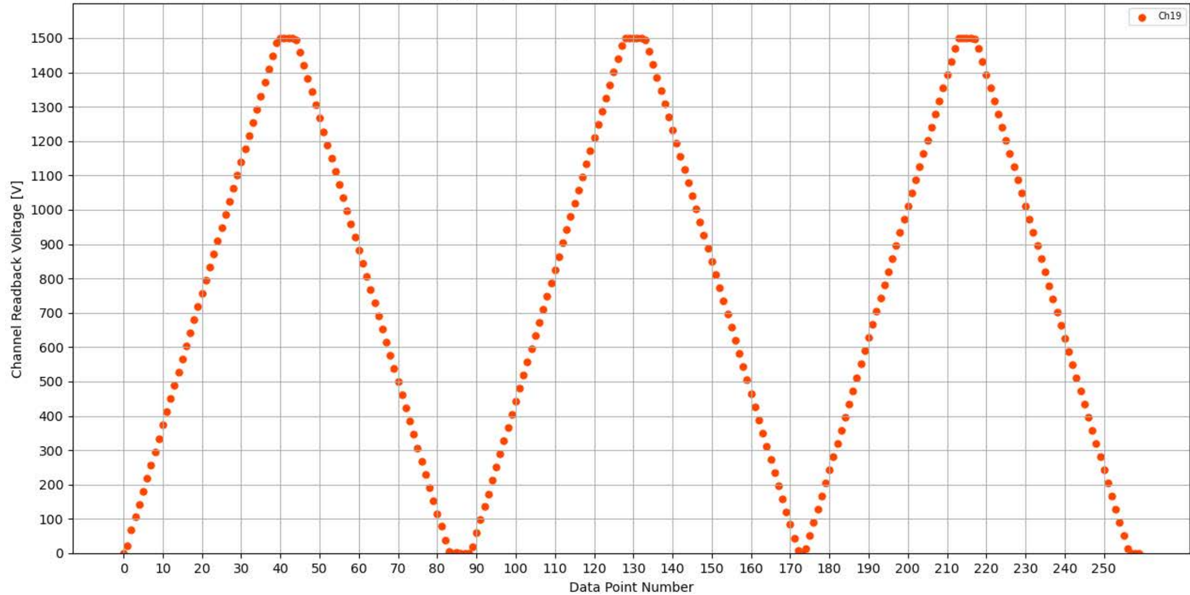
Voltage Ramp Test (Python) Bd #347, Slot #13, Ch #19
