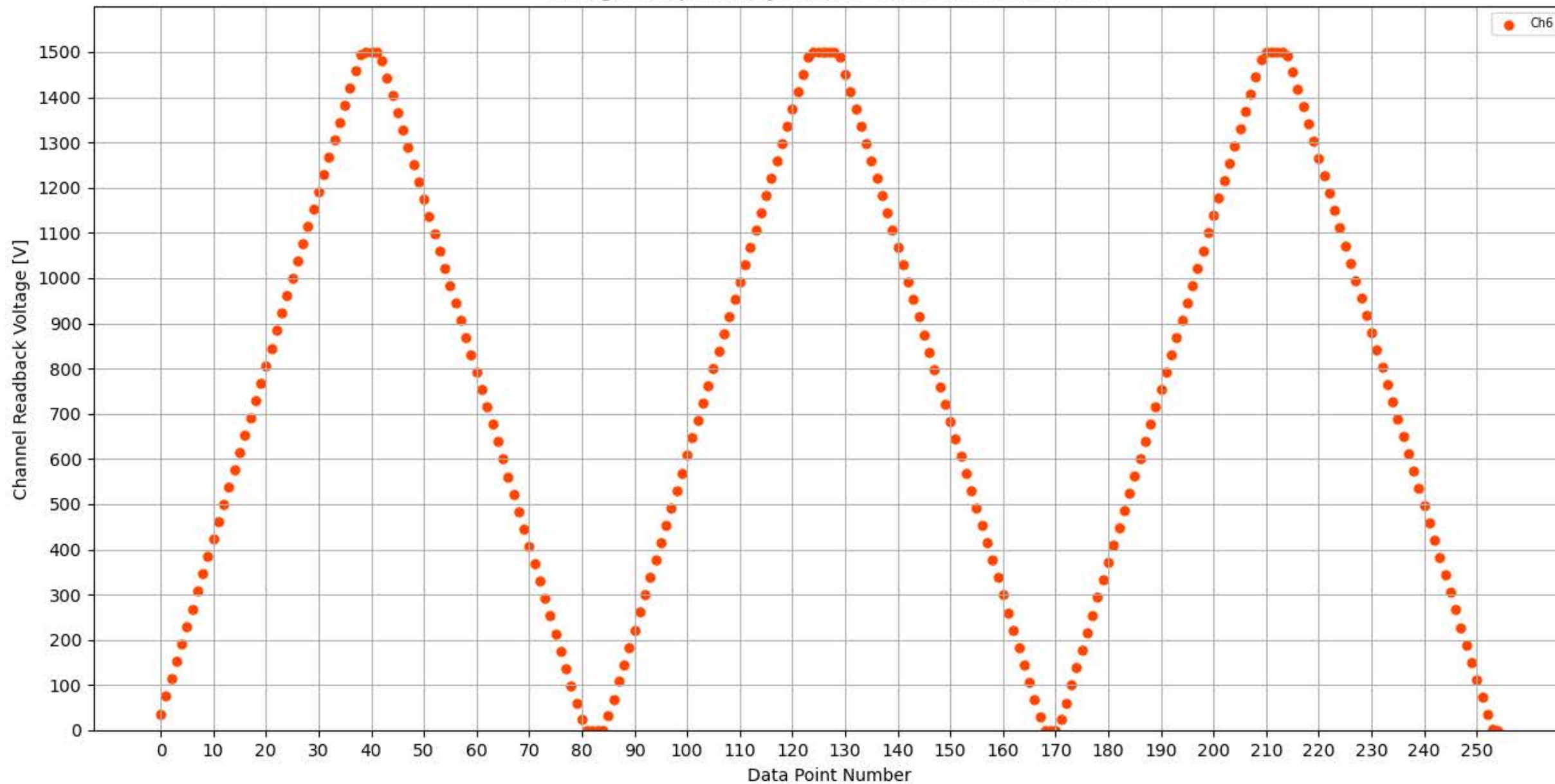
Voltage Ramp Test (Python) Bd #347, Slot #13, Ch #6
