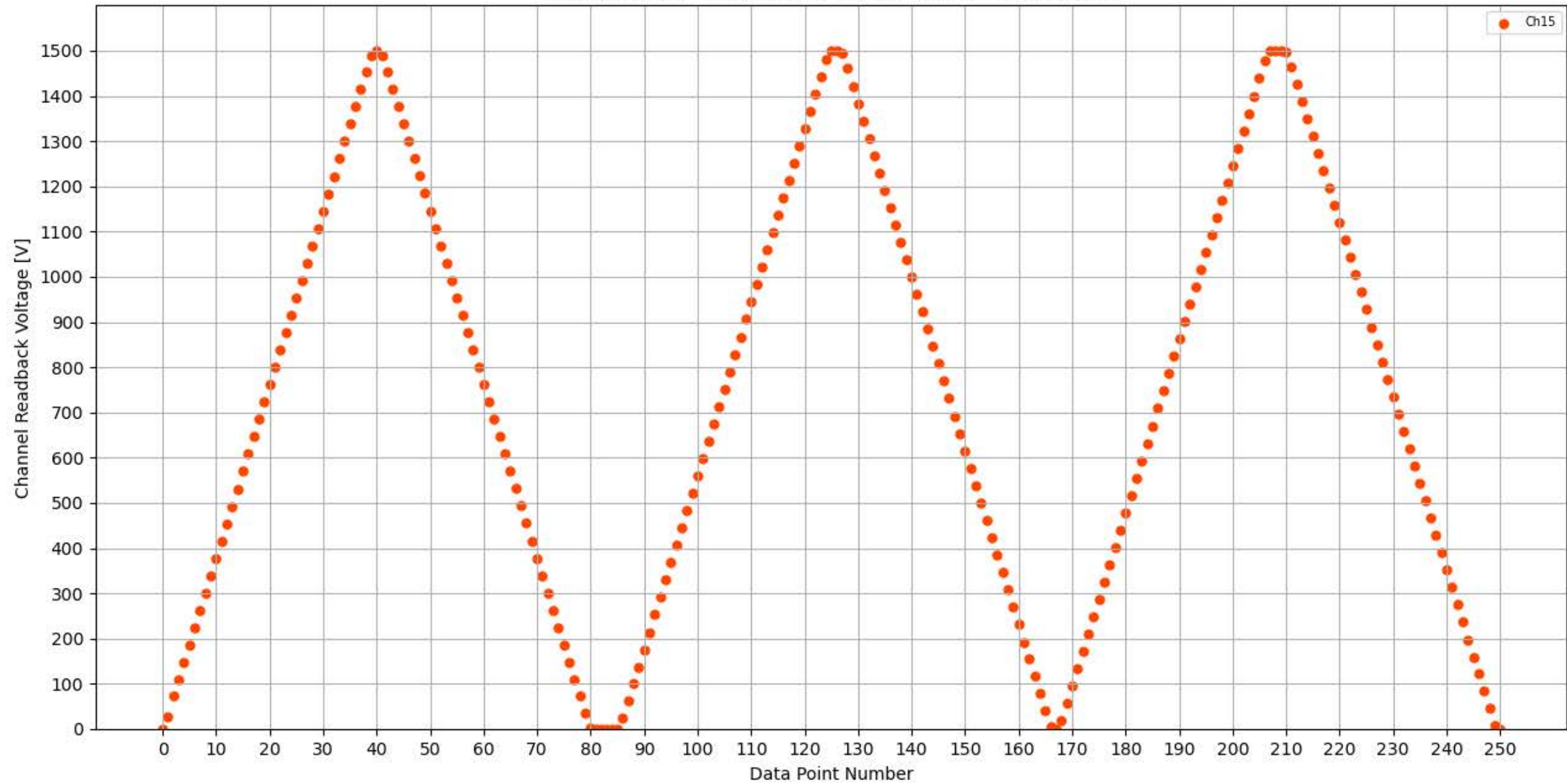
Voltage Ramp Test (Python) Bd #347, Slot #13, Ch #15
