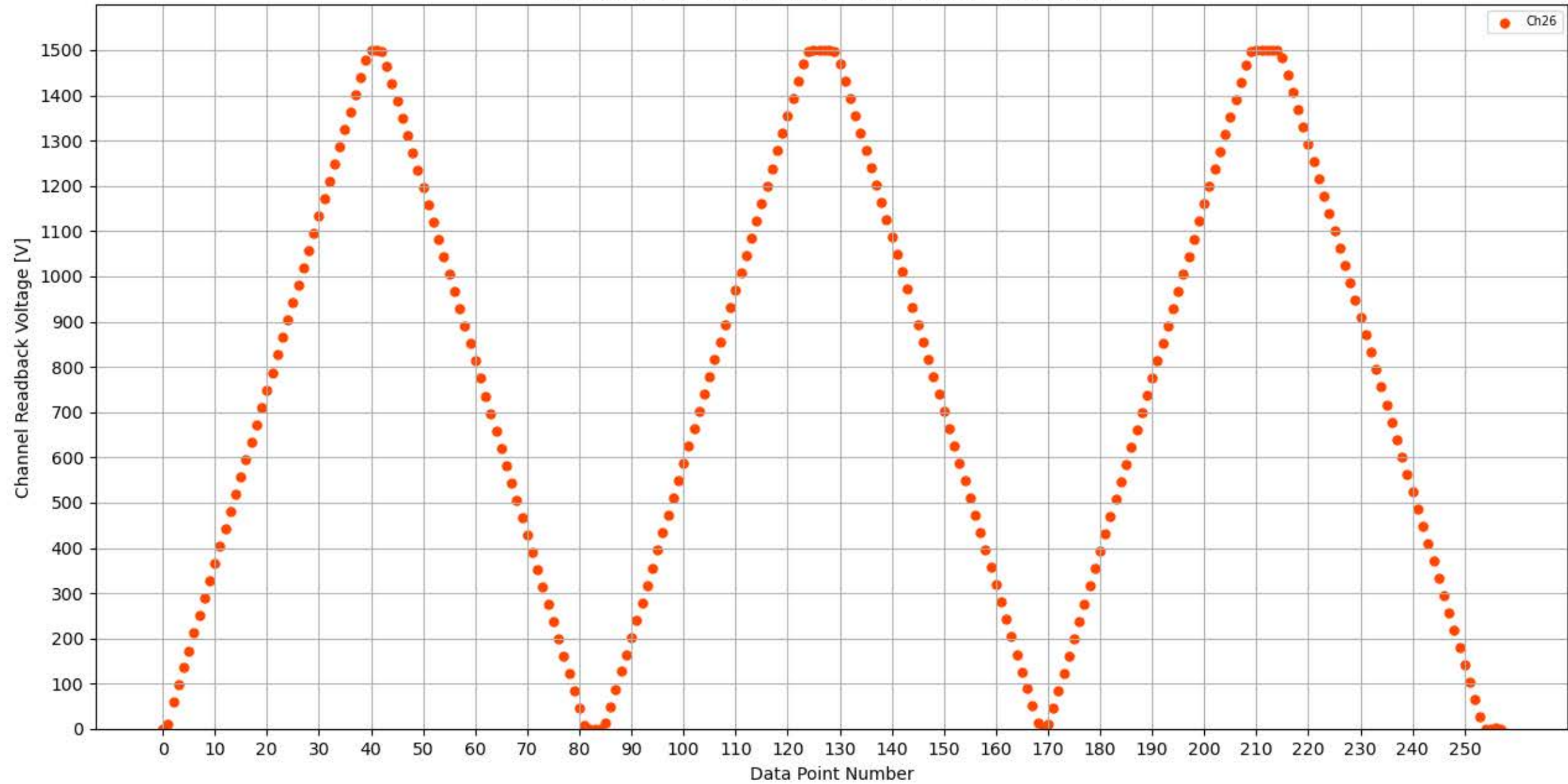
Voltage Ramp Test (Python) Bd #347, Slot #13, Ch #26
