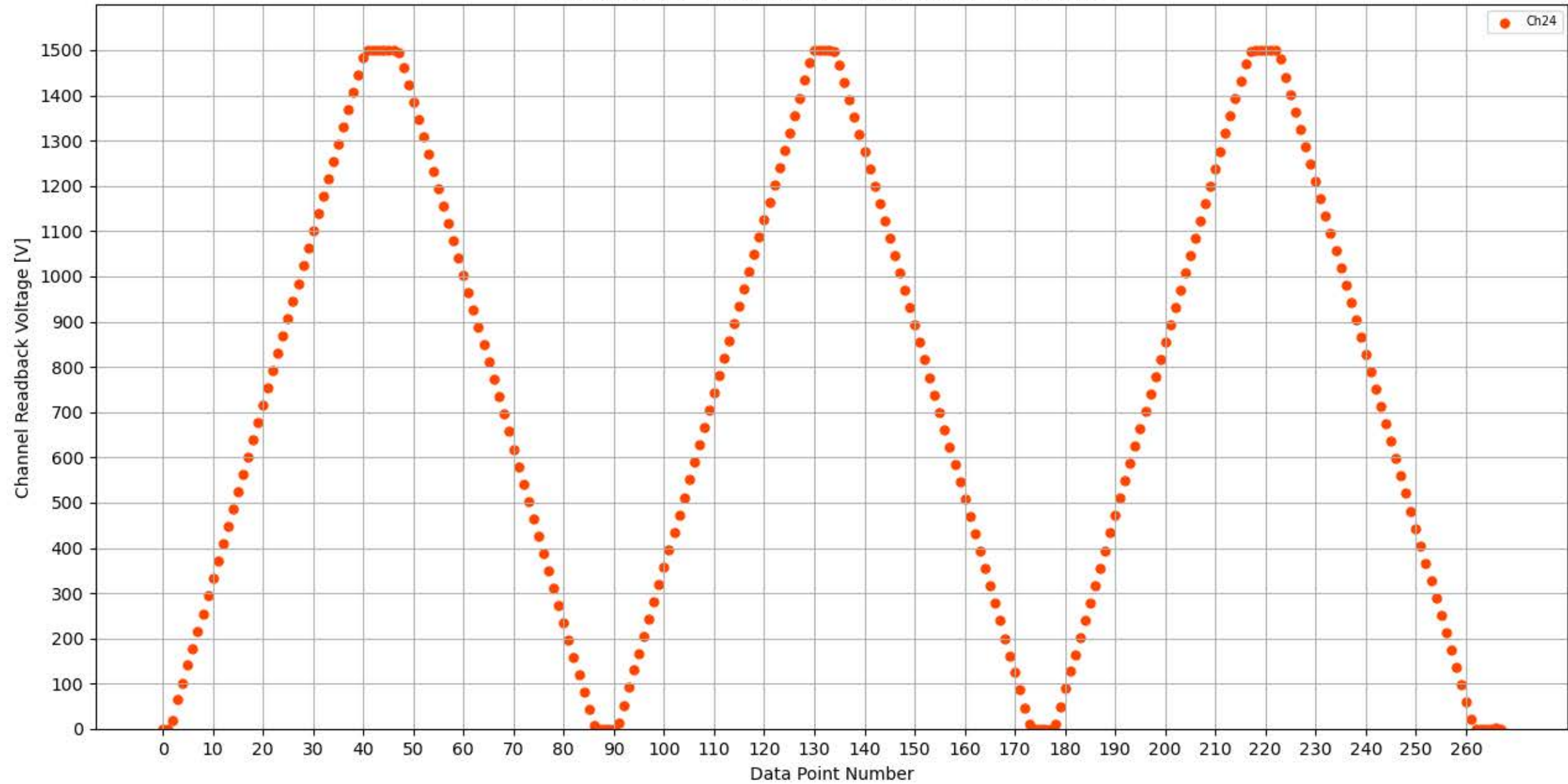
Voltage Ramp Test (Python) Bd #347, Slot #13, Ch #24
