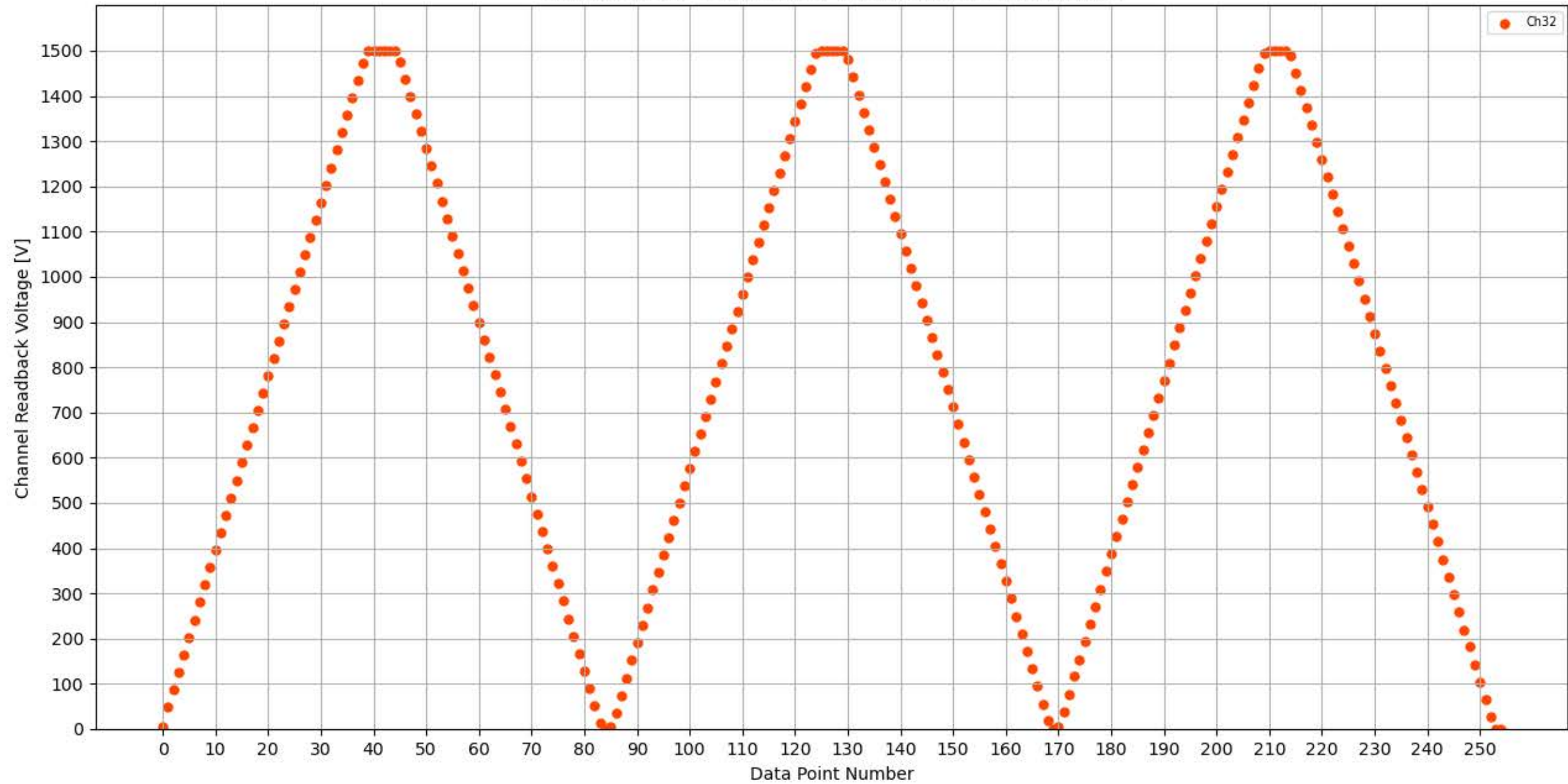
Voltage Ramp Test (Python) Bd #347, Slot #13, Ch #32
