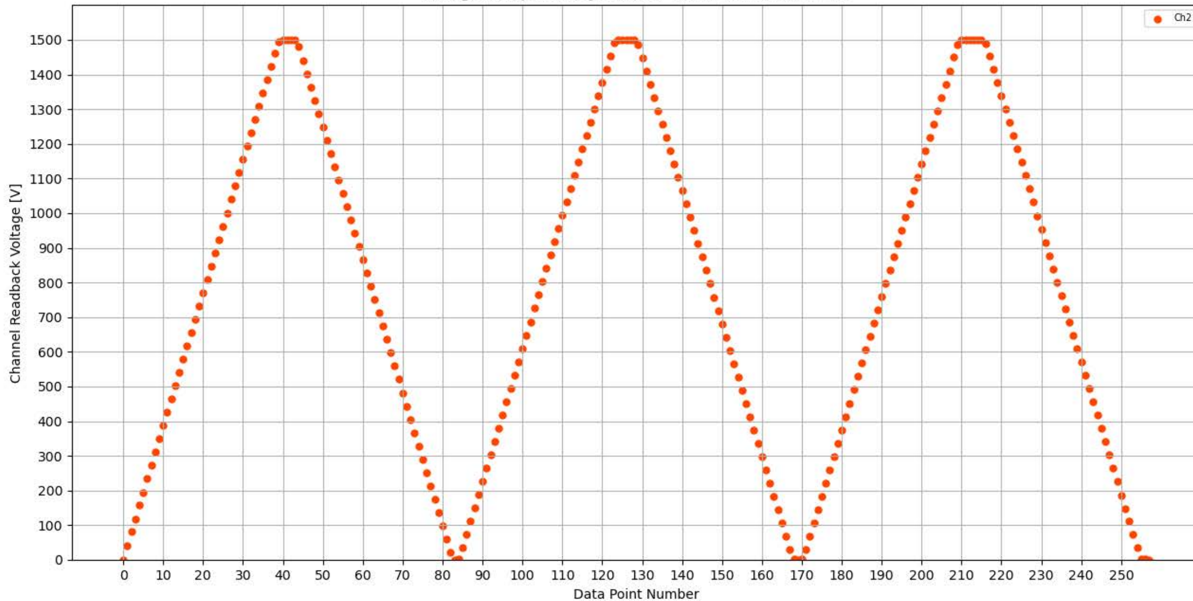
Voltage Ramp Test (Python) Bd #347, Slot #13, Ch #2
