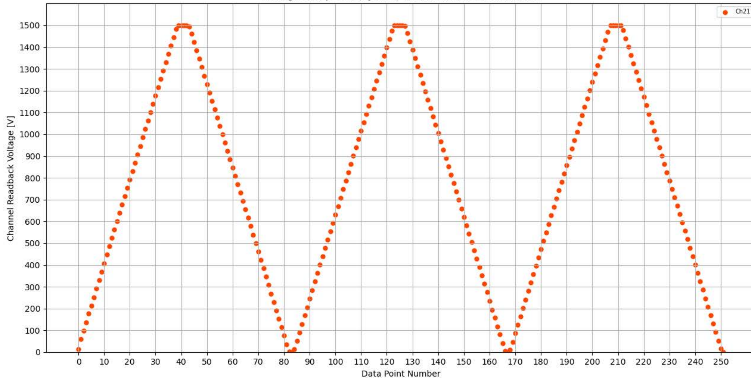
Voltage Ramp Test (Python) Bd #347, Slot #13, Ch #21
