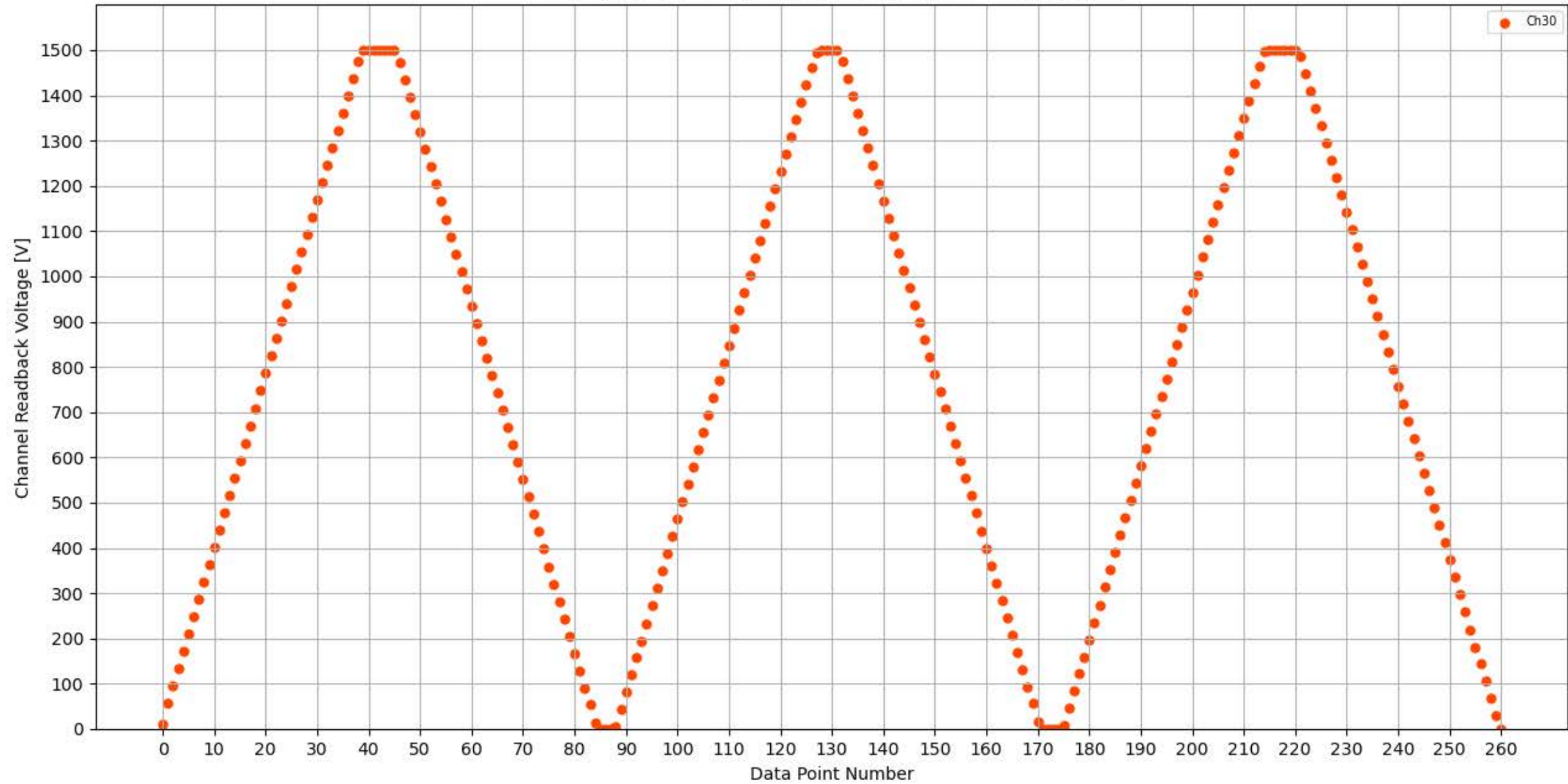
Voltage Ramp Test (Python) Bd #347, Slot #13, Ch #30
