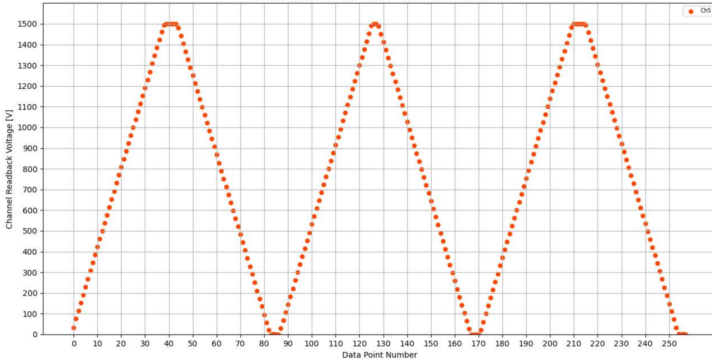
Voltage Ramp Test (Python) Bd #347, Slot #13, Ch #5
