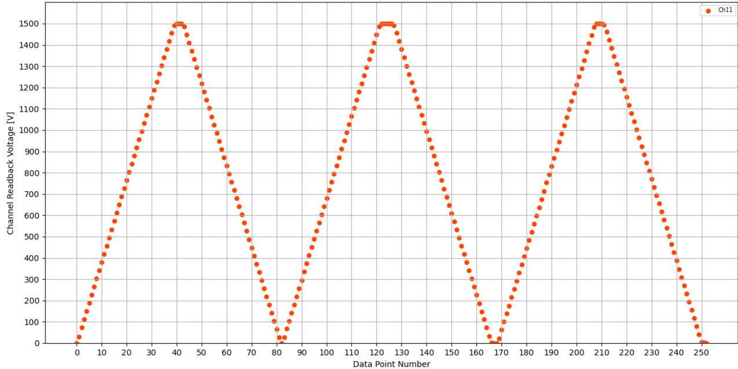
Voltage Ramp Test (Python) Bd #347, Slot #13, Ch #11
