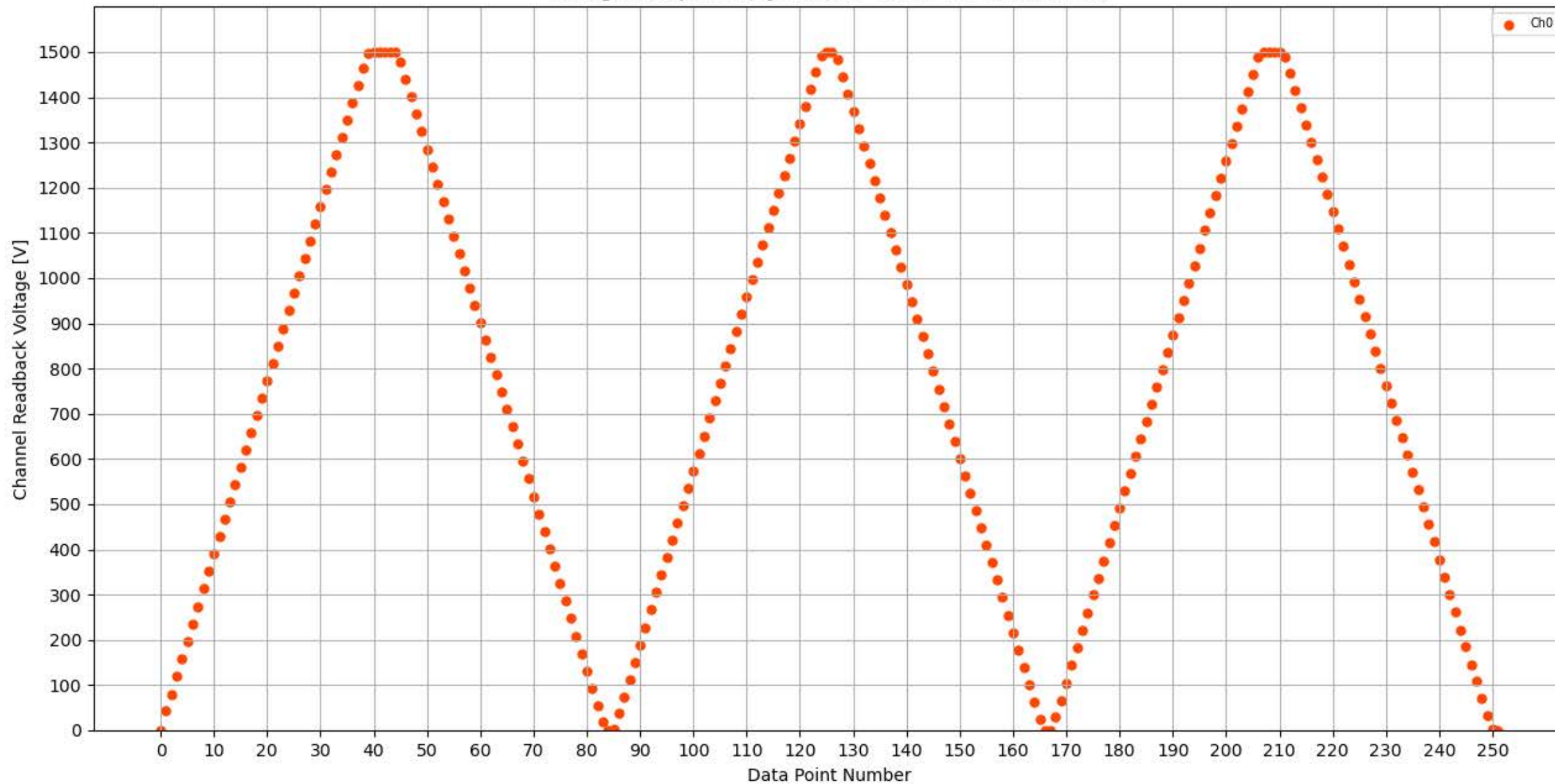
Voltage Ramp Test (Python) Bd #347, Slot #13, Ch #0
