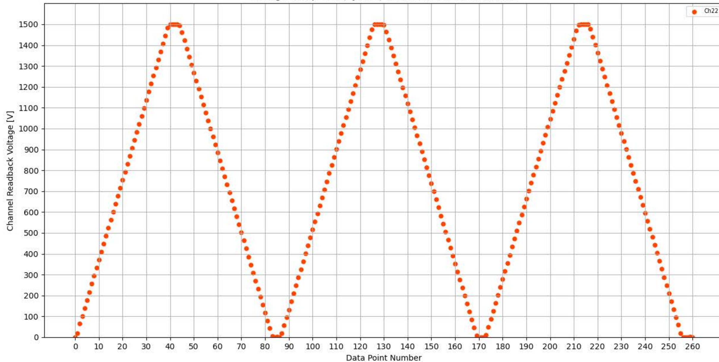
Voltage Ramp Test (Python) Bd #347, Slot #13, Ch #22
