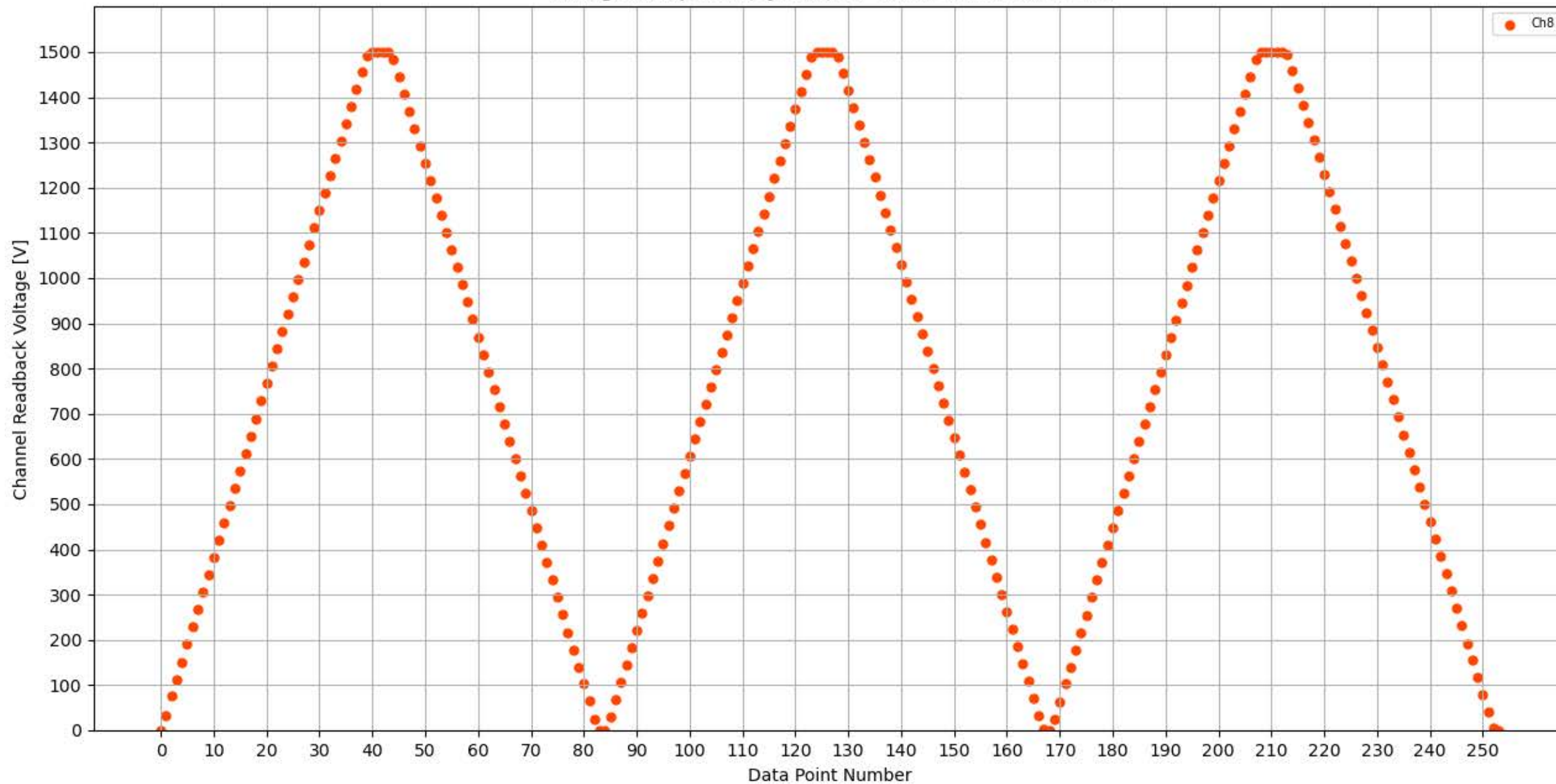
Voltage Ramp Test (Python) Bd #347, Slot #13, Ch #8
