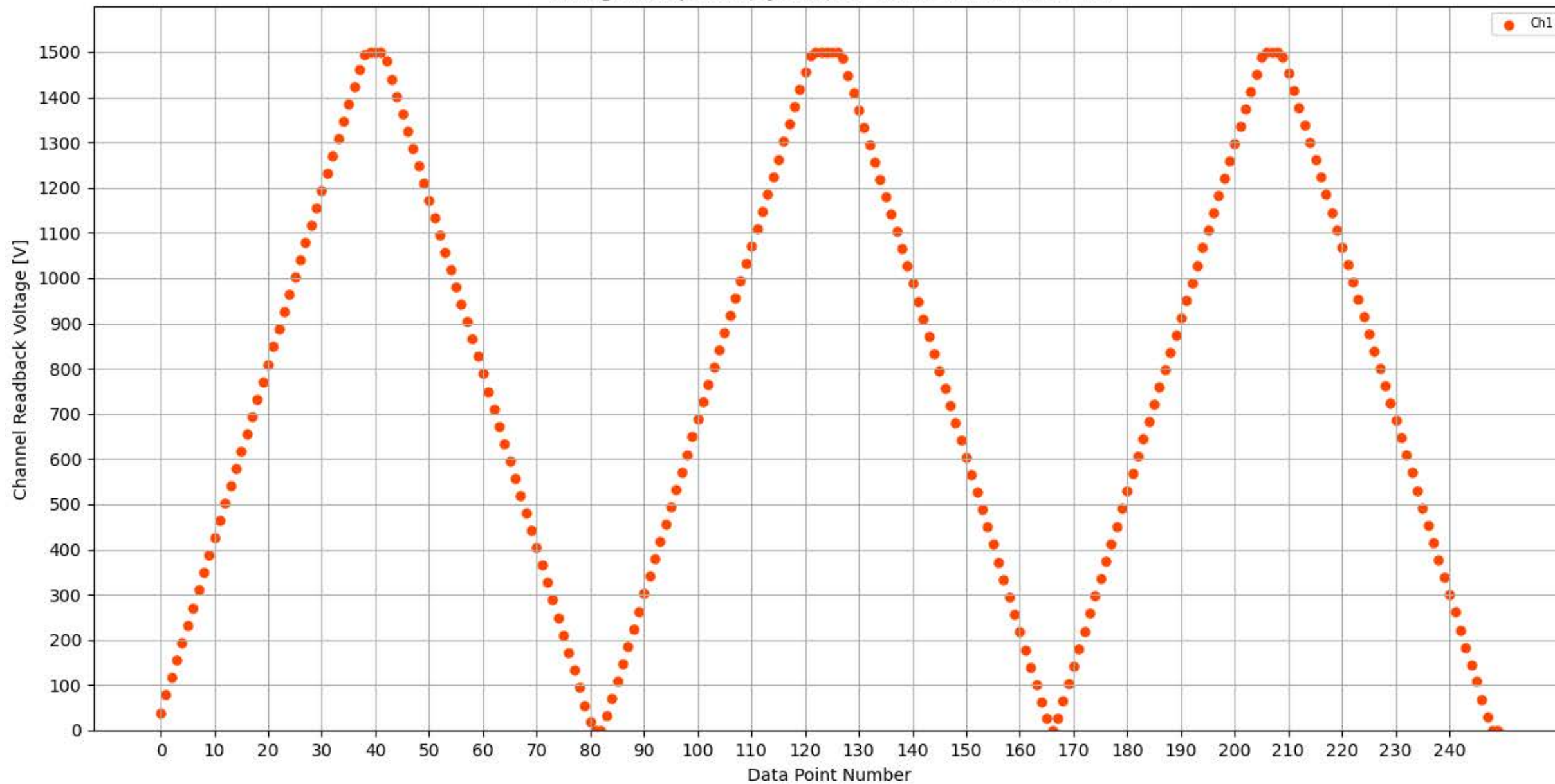
Voltage Ramp Test (Python) Bd #347, Slot #13, Ch #1
