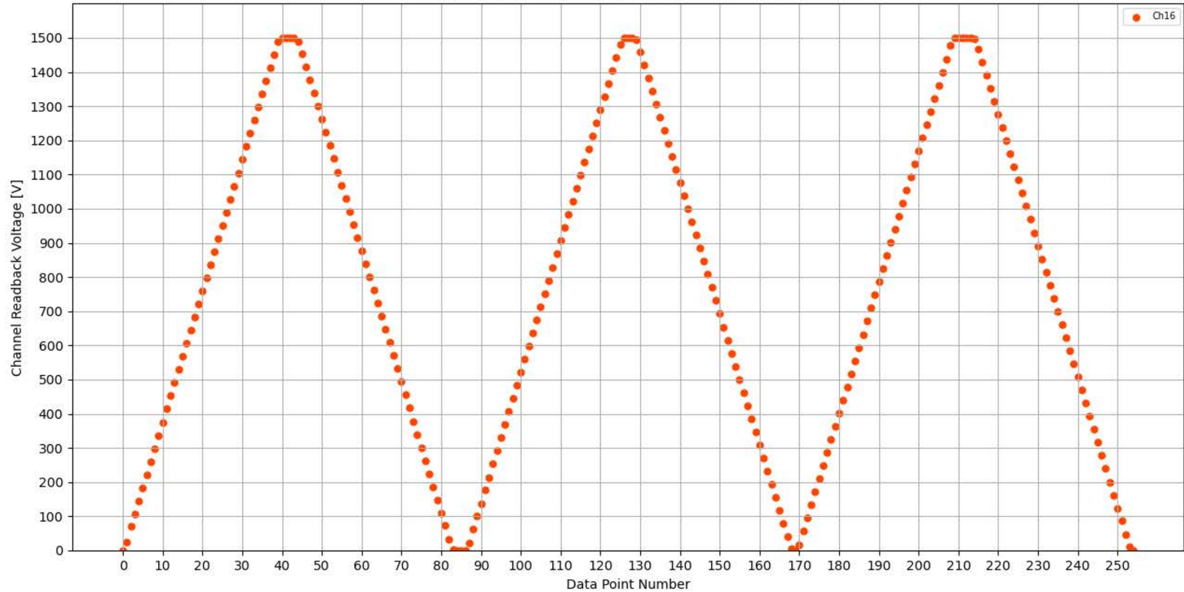
Voltage Ramp Test (Python) Bd #347, Slot #13, Ch #16
