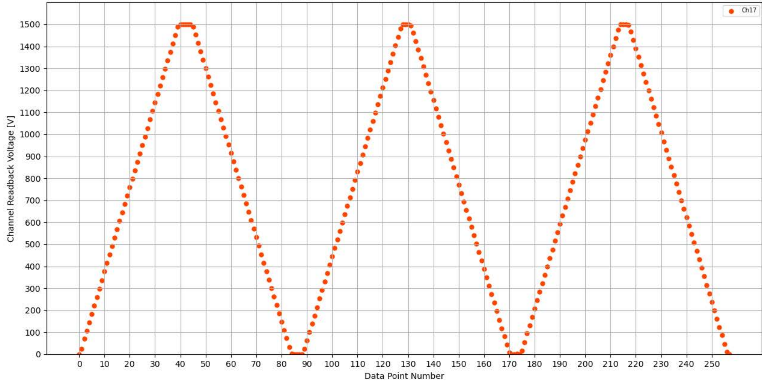
Voltage Ramp Test (Python) Bd #347, Slot #13, Ch #17
