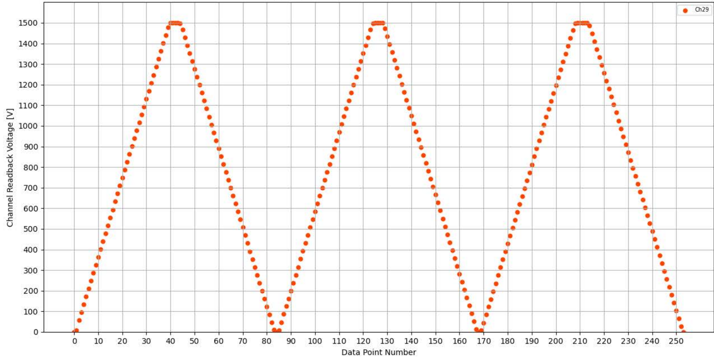
Voltage Ramp Test (Python) Bd #347, Slot #13, Ch #29
