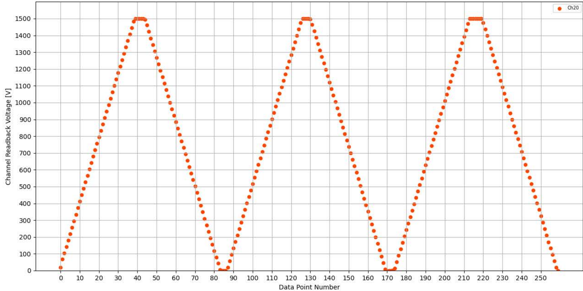
Voltage Ramp Test (Python) Bd #347, Slot #13, Ch #20
