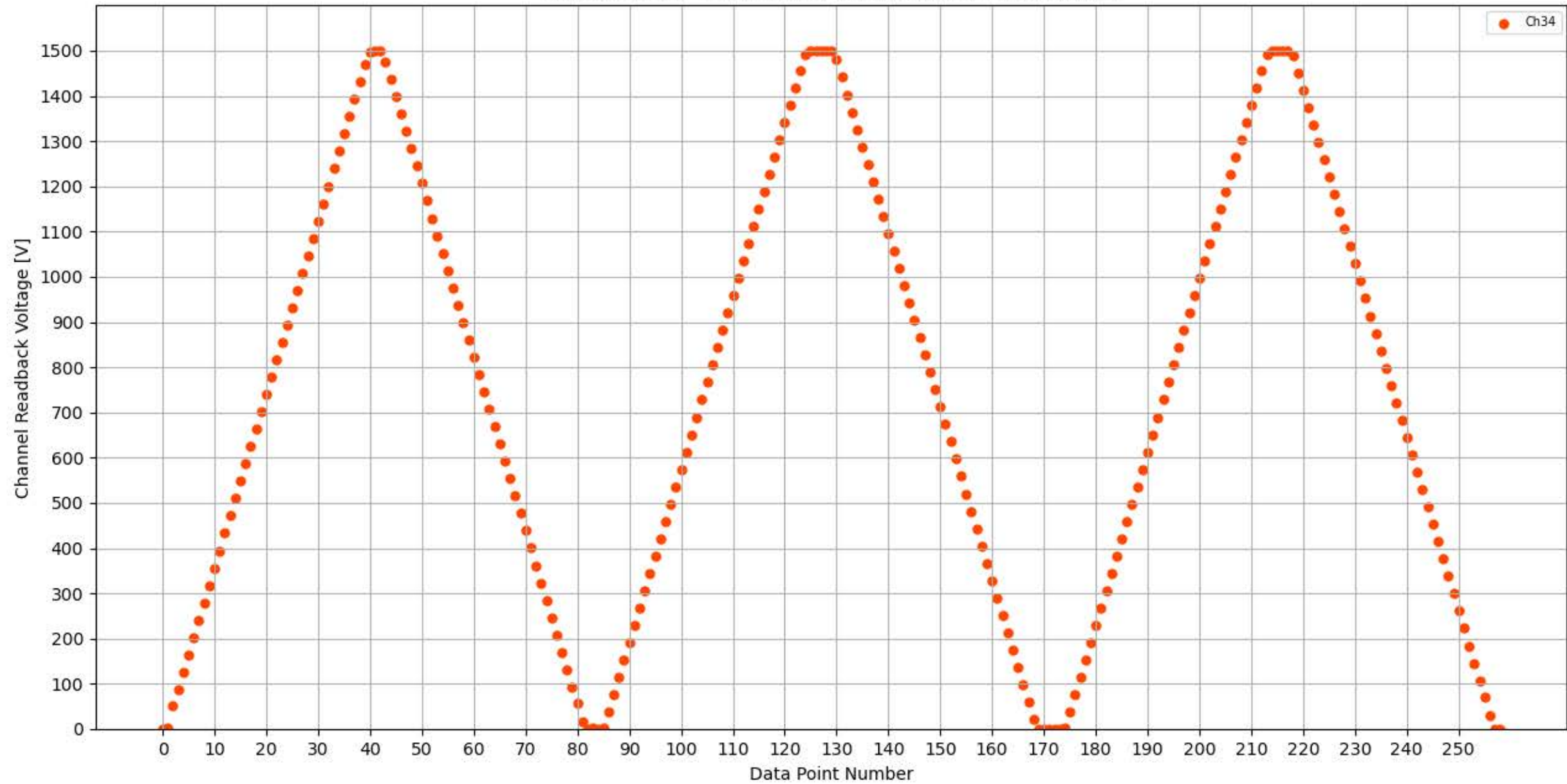
Voltage Ramp Test (Python) Bd #347, Slot #13, Ch #34
