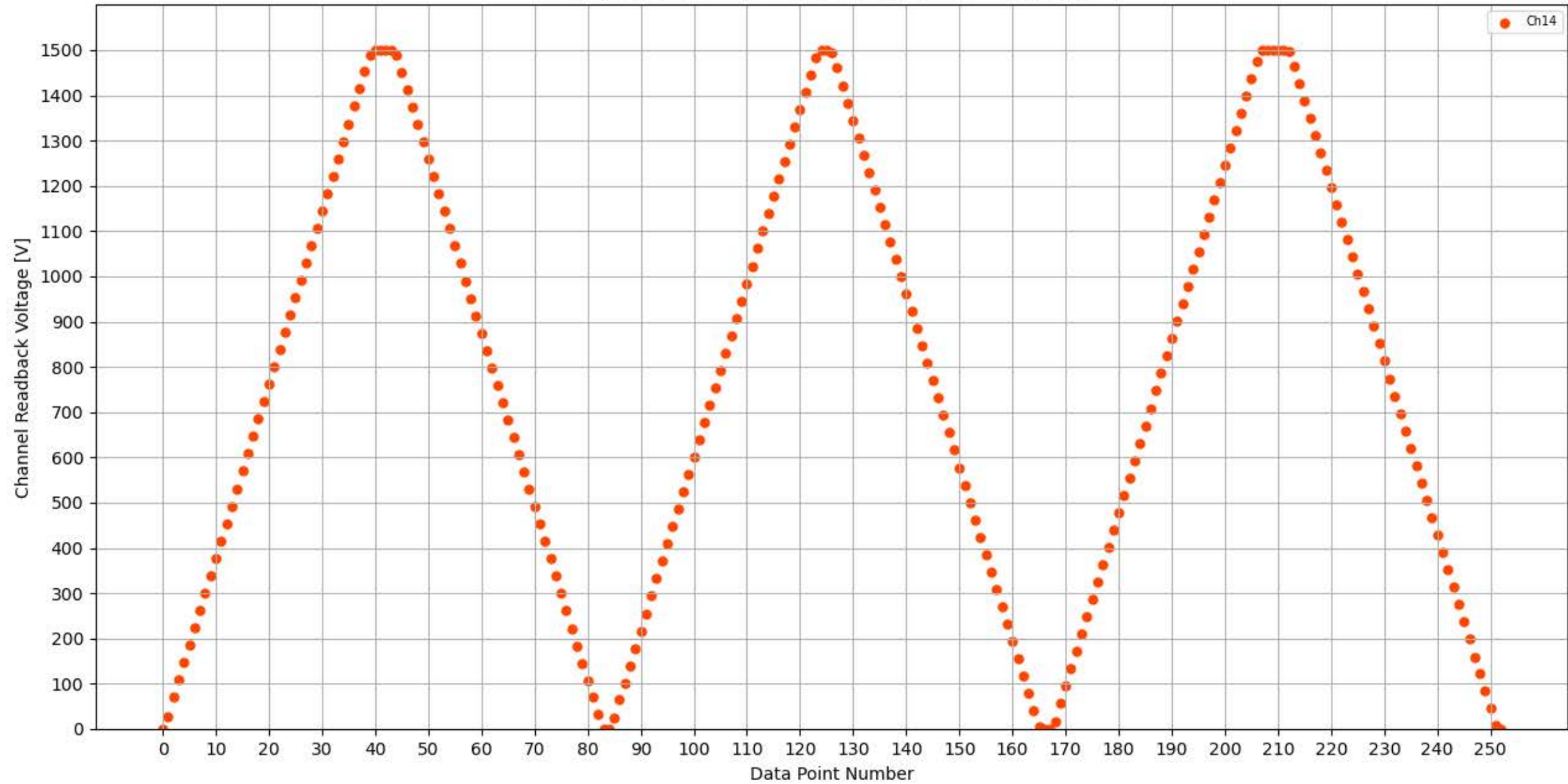
Voltage Ramp Test (Python) Bd #347, Slot #13, Ch #14
