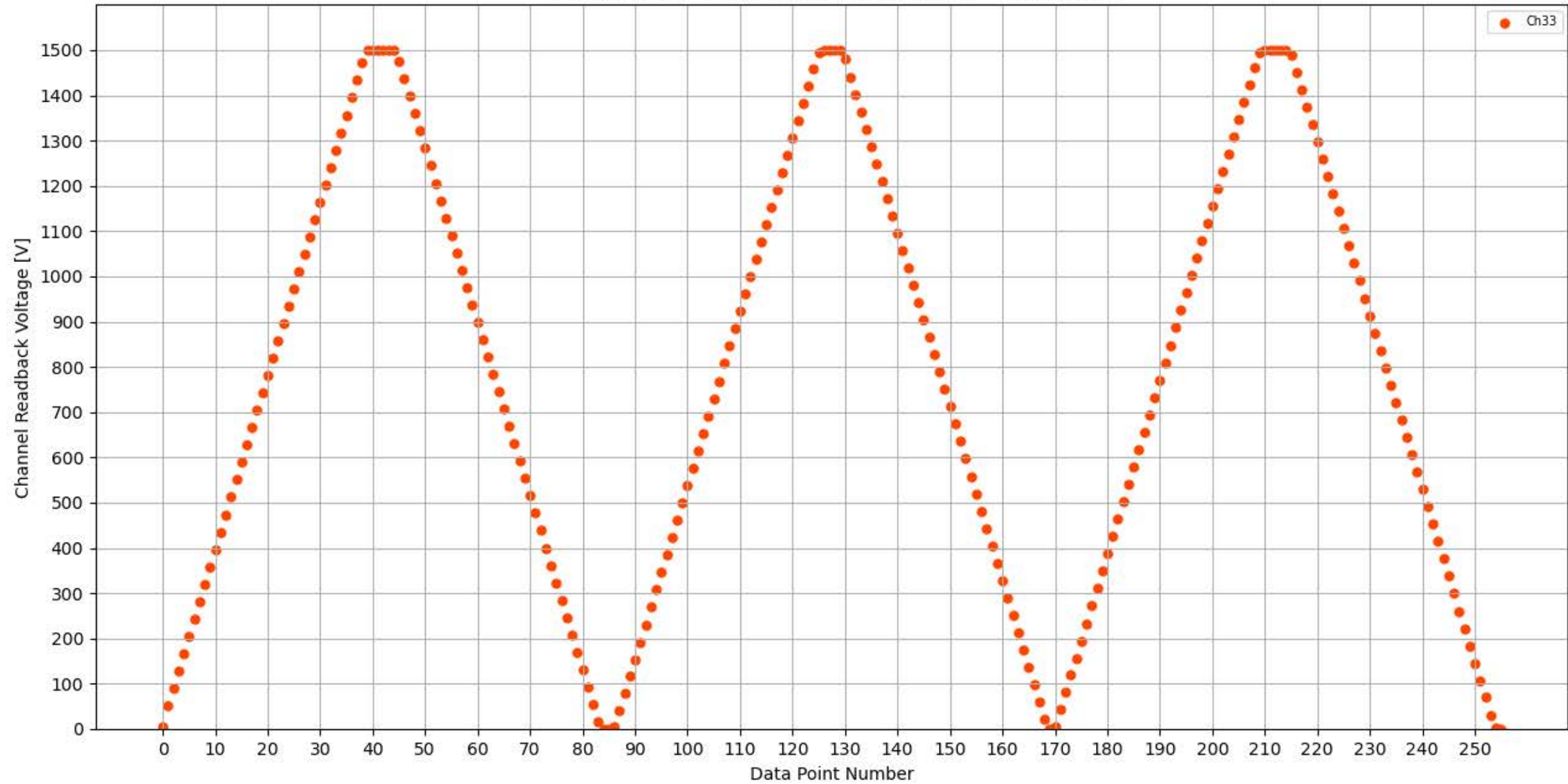
Voltage Ramp Test (Python) Bd #347, Slot #13, Ch #33
