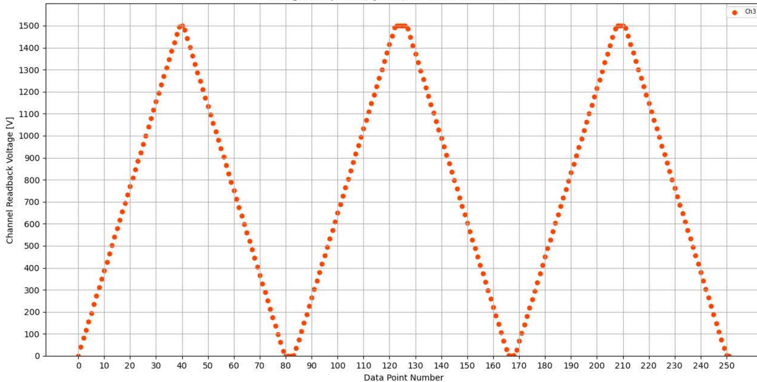
Voltage Ramp Test (Python) Bd #347, Slot #13, Ch #3
