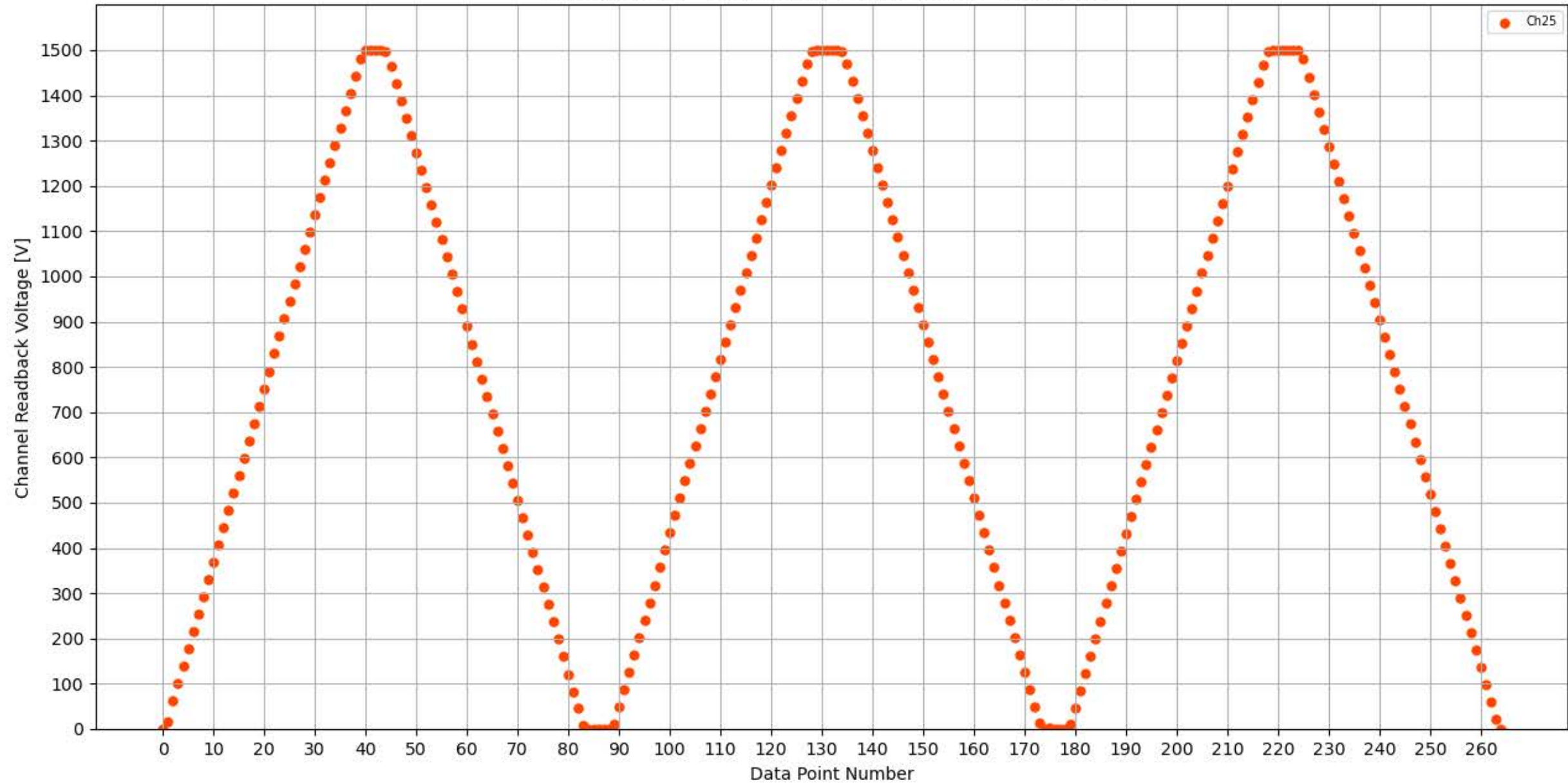
Voltage Ramp Test (Python) Bd #347, Slot #13, Ch #25
