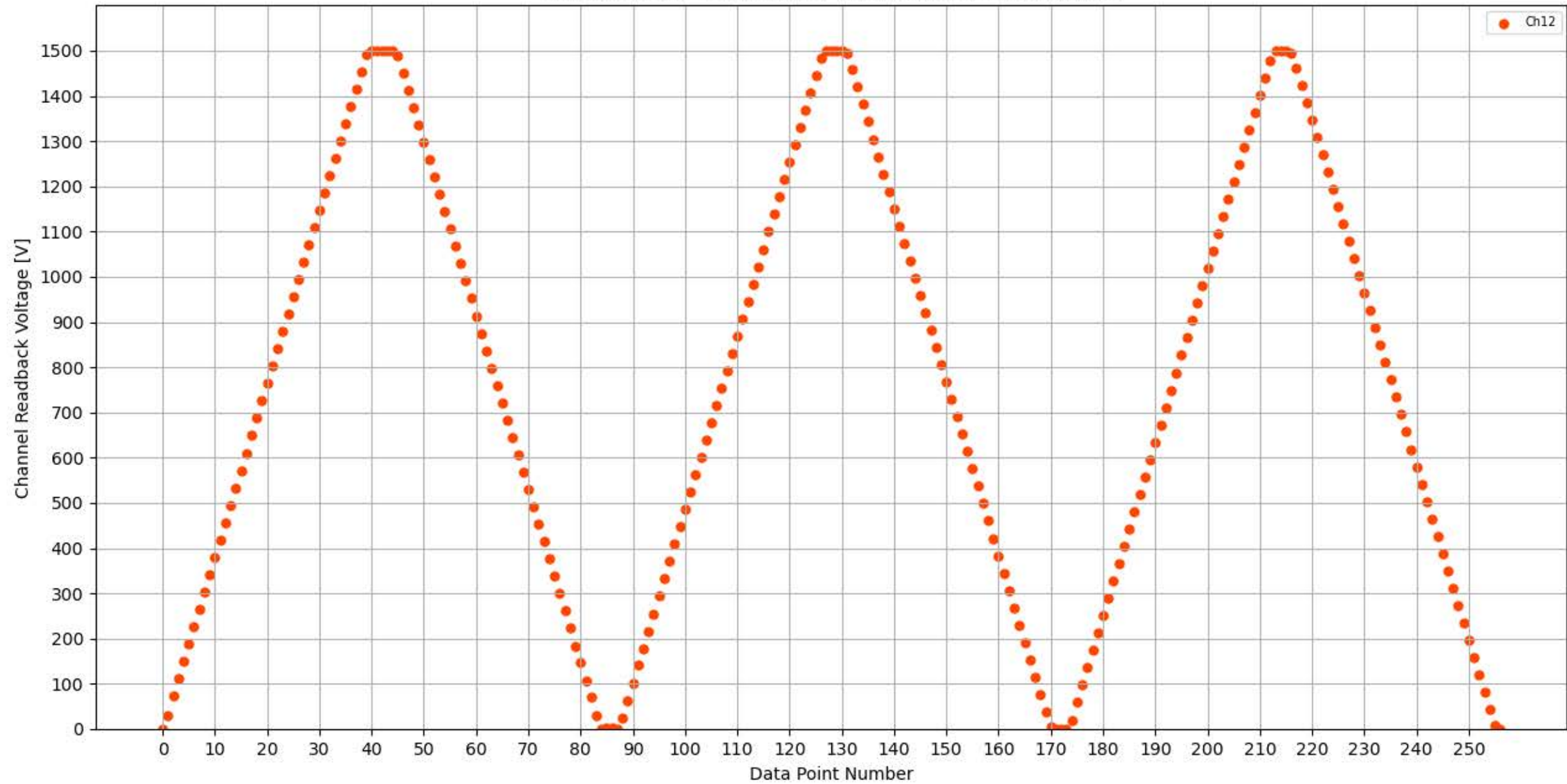
Voltage Ramp Test (Python) Bd #347, Slot #13, Ch #12
