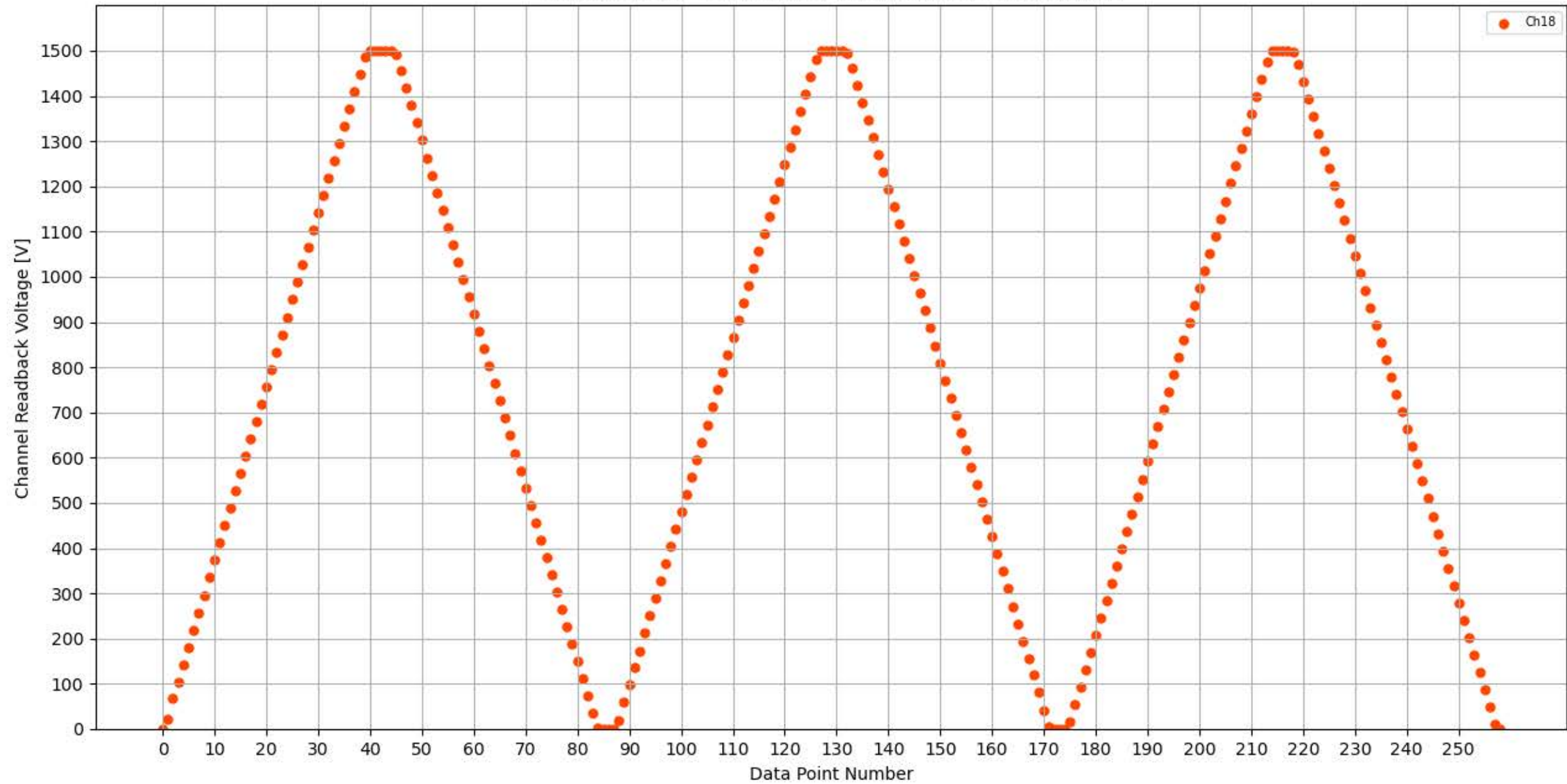
Voltage Ramp Test (Python) Bd #347, Slot #13, Ch #18
